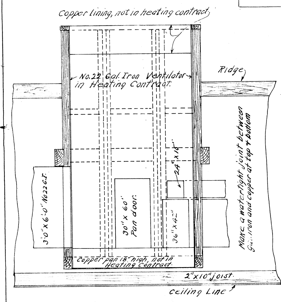
SECTION X. Y. Scale 1/4" = 1'-0"
